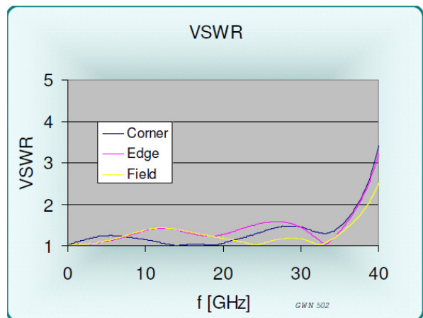
Figure 4: VSWR, AA917-E5
