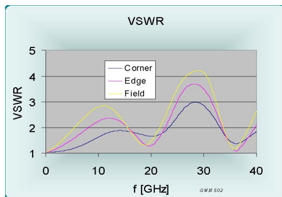
Figure 4: VSWR, B2500-K2
