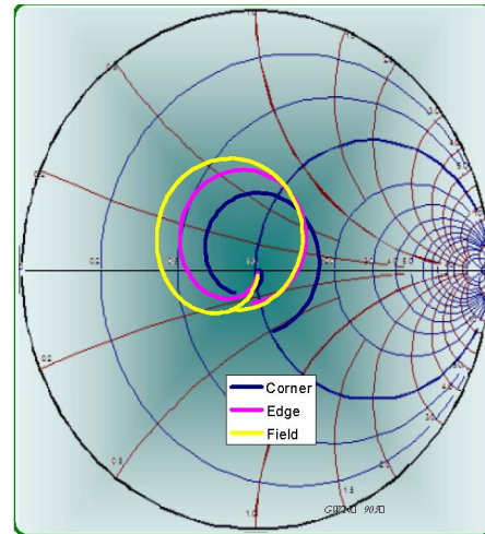
Figure 2: Measurement into 50Ω, B2500-K2
