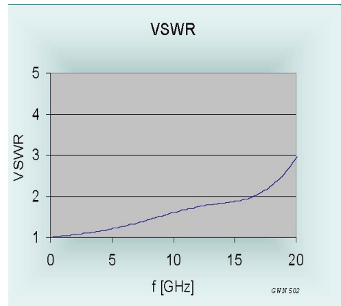
Figure 2: VSWR, B2504-C3
