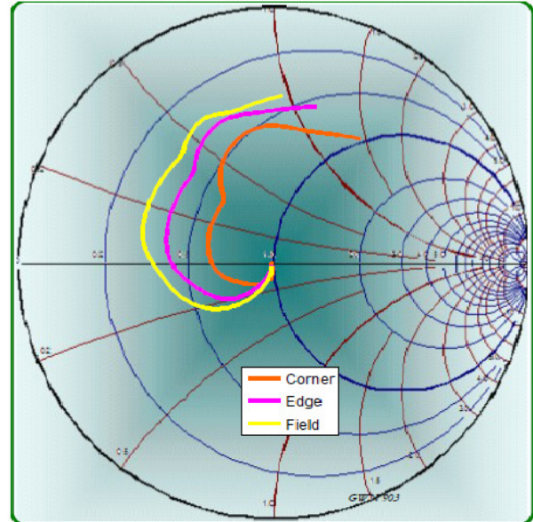
Figure 2: Measurement into 50Ω, B2509-F6
