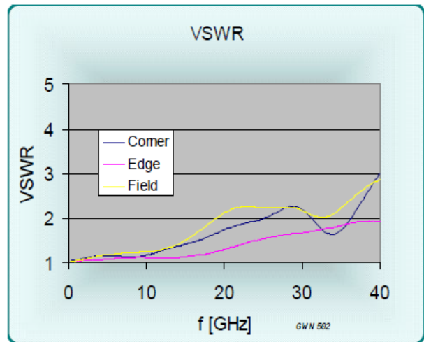
Figure 4: VSWR, D4595-B2
