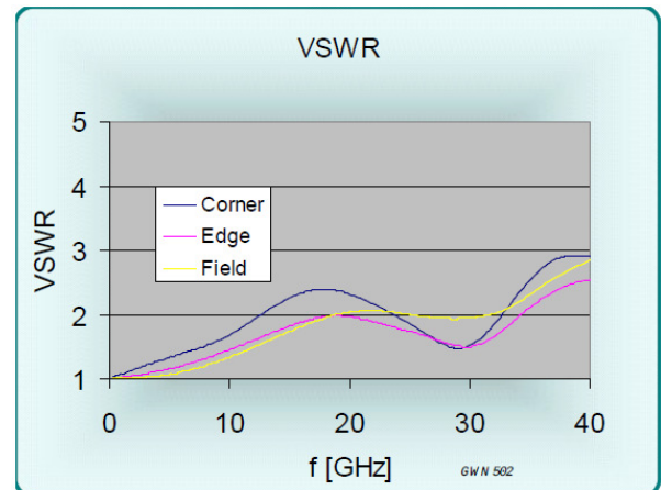
Figure 4: VSWR, D4595-B2
