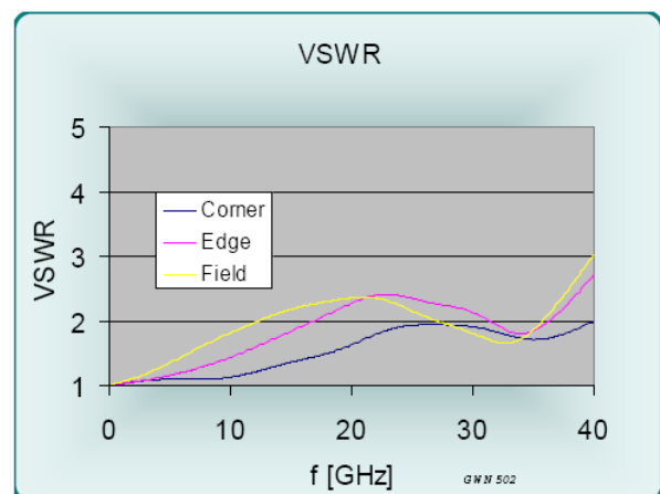
Figure 4: VSWR, E5656-B2
