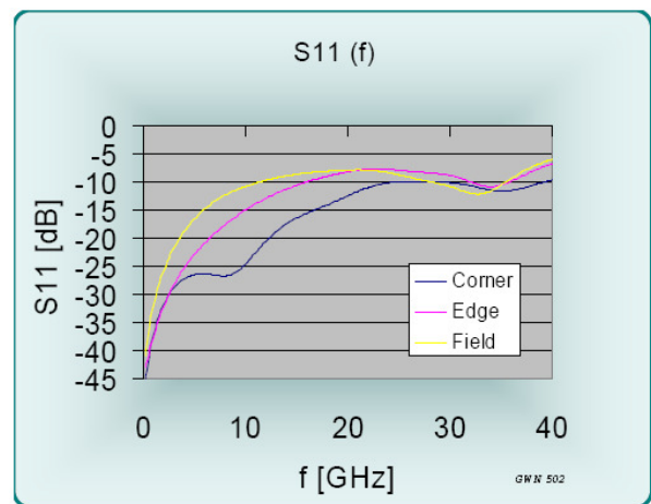
Figure 3: Return Loss, S11, E5656-B2
